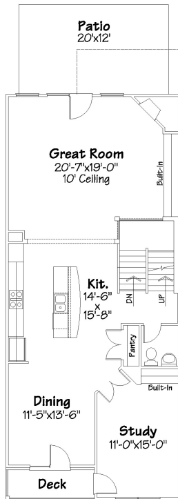
FIRST FLOOR PLAN 1226 SQ. FT.
