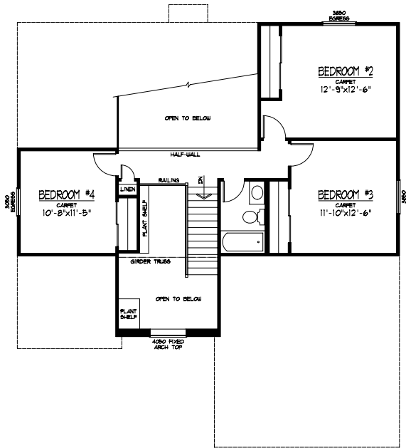
SECOND FLOOR PLAN SCALE: 1/8"=1'-0" 665 SQ FT
