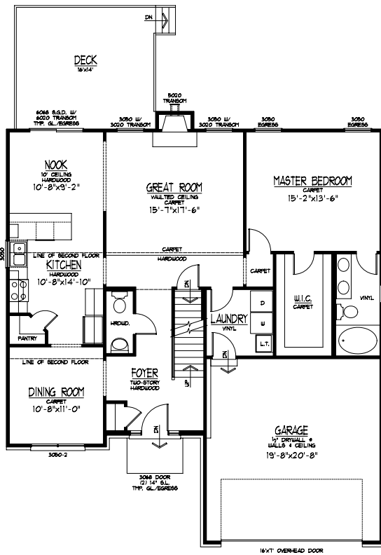
FIRST FLOOR PLAN SCALE: 1/8"=1'-0" 1338 SQ FT
